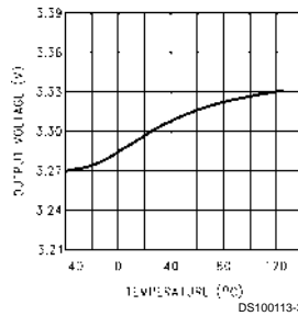
Output Voltage vs Temperature (3.3V)
