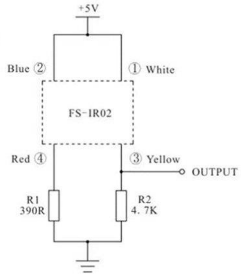
DC5V typical application circuit
