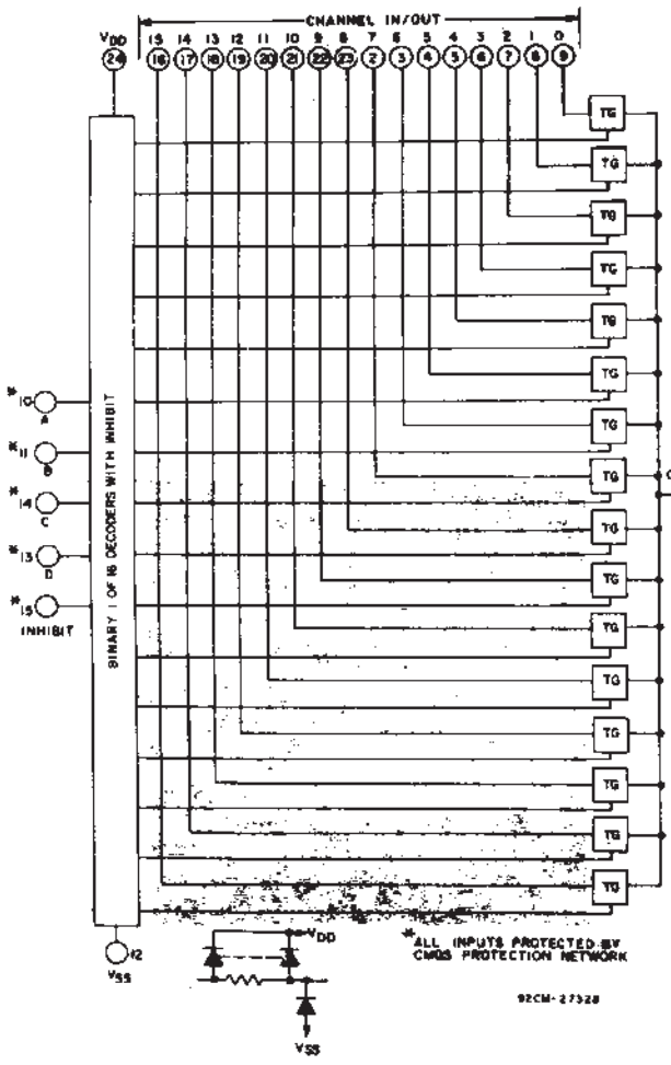
Fig. 16- CD4067 logic diagram.
