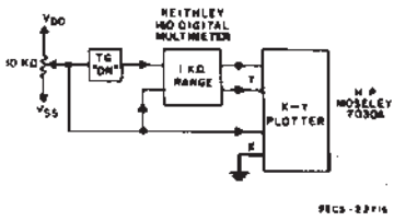
Fig. 13- Channel ON resistance measurement circuit.
