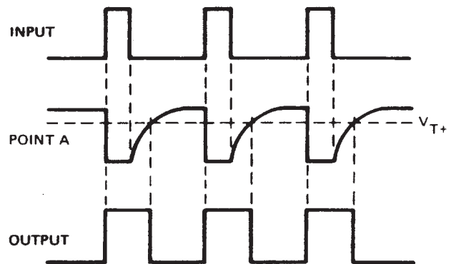
PULSE STRETCHER
