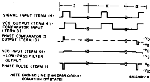
Fig. 10 - Typical waveforms for CMOS/MOS phase-locked loop employing phase comparator II in locked condition.
