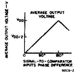
Fig. 2 - Phase-comparator I characteristics at low-pass filter output.
