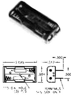
CAT. NO. 2468 – PC Mount CAT. NO. 2469 – 6" Wire Leads
