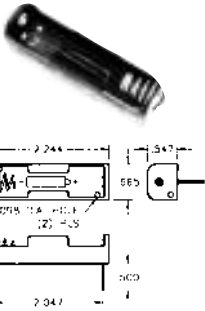
CAT. NO. 2460 – PC Mount CAT. NO. 2461 – 6" Wire Leads
