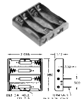
CAT. NO. 2481 – PC Mount CAT. NO. 2482 – 6" Wire Leads
