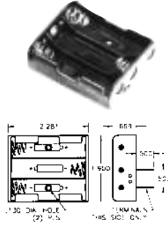
CAT. NO. 2464 – PC Mount CAT. NO. 2465 – 6" Wire Leads
